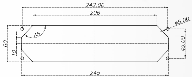
TTB DIMENSION AND PANEL CUTOUT
