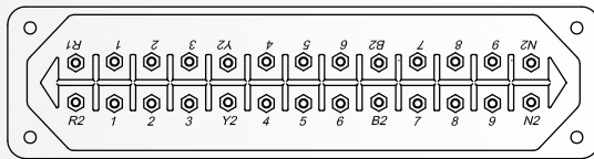
REAR VIEW TERMINAL DETAILS
