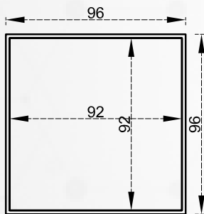
PANEL CUTOUT - 92X92 mm BEZZEL - 96X96 mm
