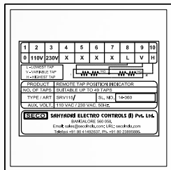
TERMINAL DETAILS
