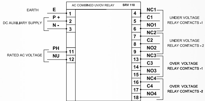
TYPICAL WIRING DIAGRAM
